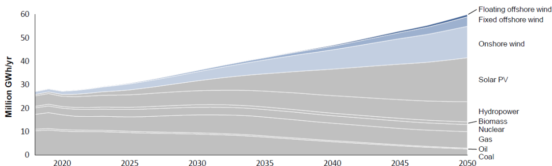
World Electricity generation – power station type
